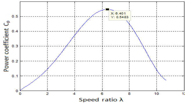
Figure 5. Characteristic of the power coefficient evolution.
