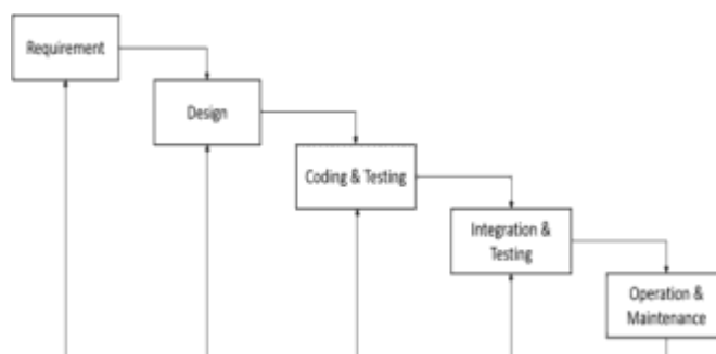
Figure 1. Waterfall method [21]
