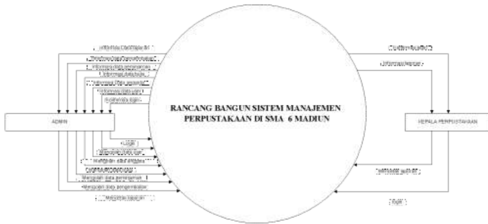
Figure 3. DFD Level 0
