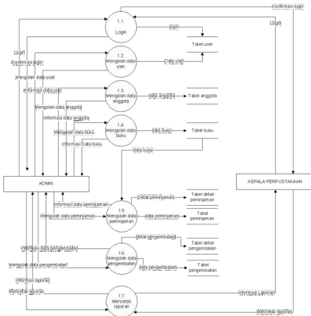
Figure 4. DFD Levels 1
