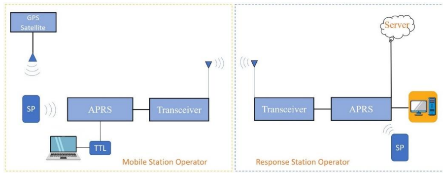
Figure 2. MSO and RSO system diagram.
