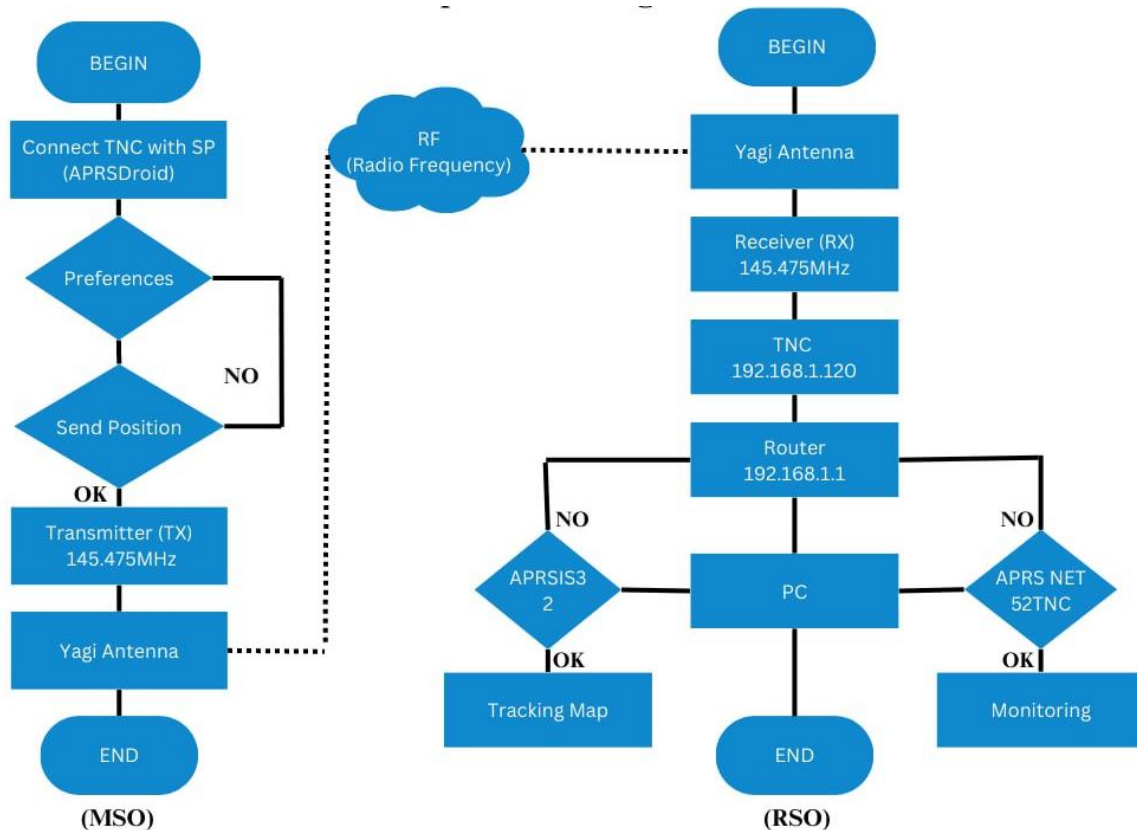
Figure 7. Experiment diagram.
