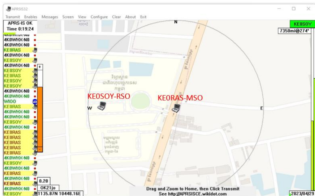
Figure 6. APRSIS application interface.
