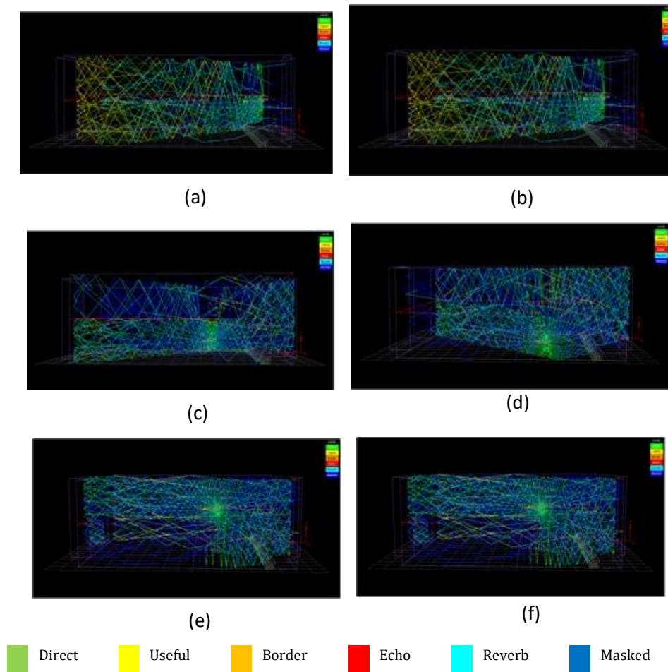
Figure 6. (a) Sound Spread Loudspeaker 1; (b) Sound Spread Loudspeaker 2; (c) Sound Spread Loudspeaker 3; (d) Sound Spread Loudspeaker 4; (e) Sound Spread Loudspeaker 5; (f) Sound Spread Loudspeaker 6.
