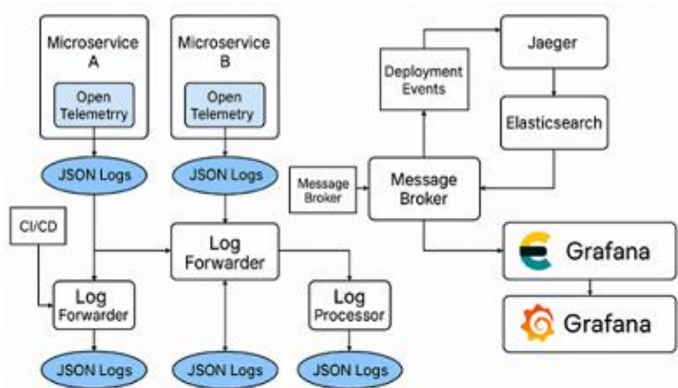
Gambar 3. API Logging integration
