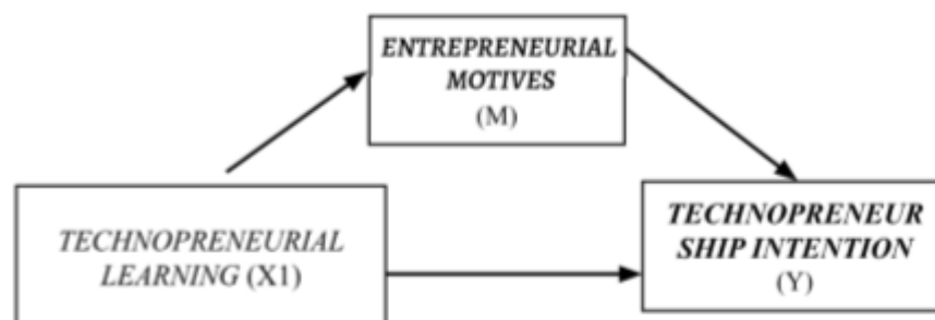
Figure 1. Theoretical Framework.
